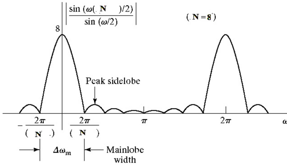
Fig. 2 : sinc-function, \Delta = 1
